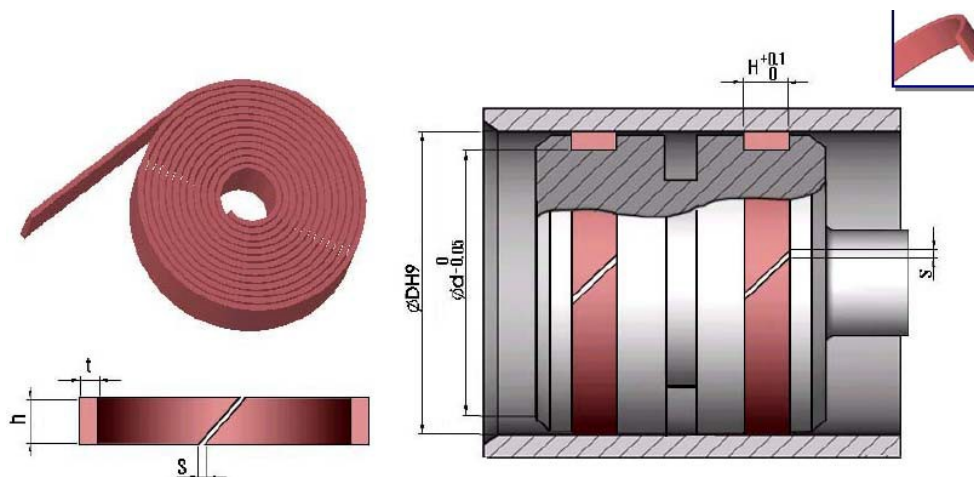
BRONZE FILLED PTFE ROLL BAND
